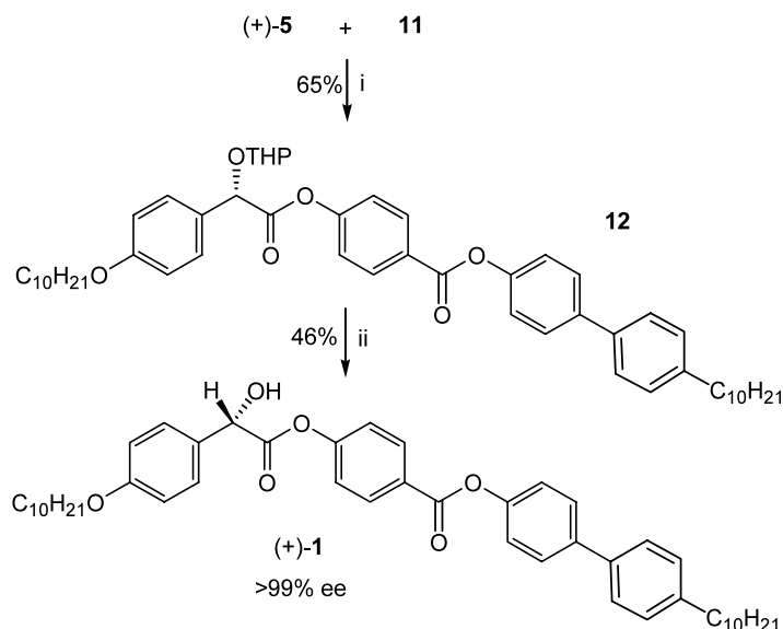
Scheme 3. Reagents and conditions: (i) (a) DHP, p -TsOH; then NaOH (1 M), (b) DCC, DMAP, THF; (ii) PPTS, wet acetone.
