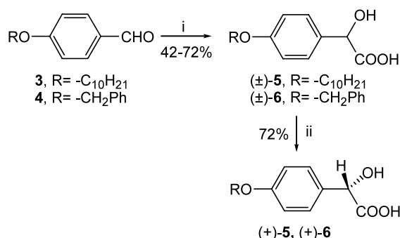
Scheme 1. Reagents and conditions: (i) CHCl 3 , NaOH (50%), BTAC; (ii) (a) ( R )-(+)-PEA, CHCl 3 , (b) HCl (2 M), Et 2 O.
