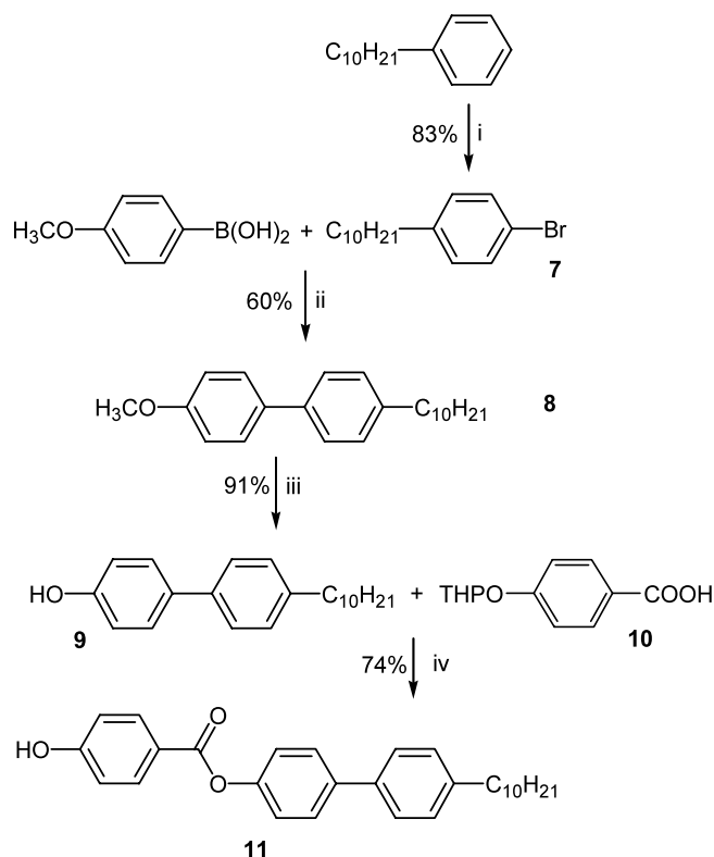
Scheme 2. Reagents and conditions: (i) Br 2 , CH 2 Cl 2 ; (ii) [Pd(PPh 3 ) 4 ], Na 2 CO 3 (2 M); (iii) BBr 3 , CH 2 Cl 2 ; (iv) (a) DCC, DMAP, THF, (b) PPTS, wet acetone.
