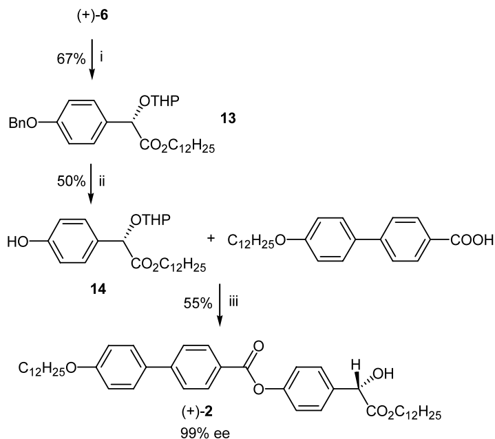
Scheme 4. Reagents and conditions: (i) (a) DHP, p -TsOH; then NaOH (1 M), (b) C 12 H 25 OH, DCC, DMAP, THF; (ii) Pd/C (10%), cyclohexene; (iii) (a) DCC, DMAP, THF, (b) PPTS, wet acetone.
